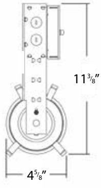
RHL4R-ICAT Remodel LED Housing
