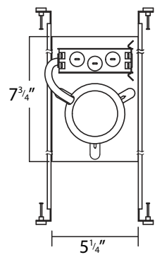
RHL4-ICAT New Construction LED Housing
