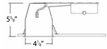
RHL4R-ICAT Remodel LED Housing
