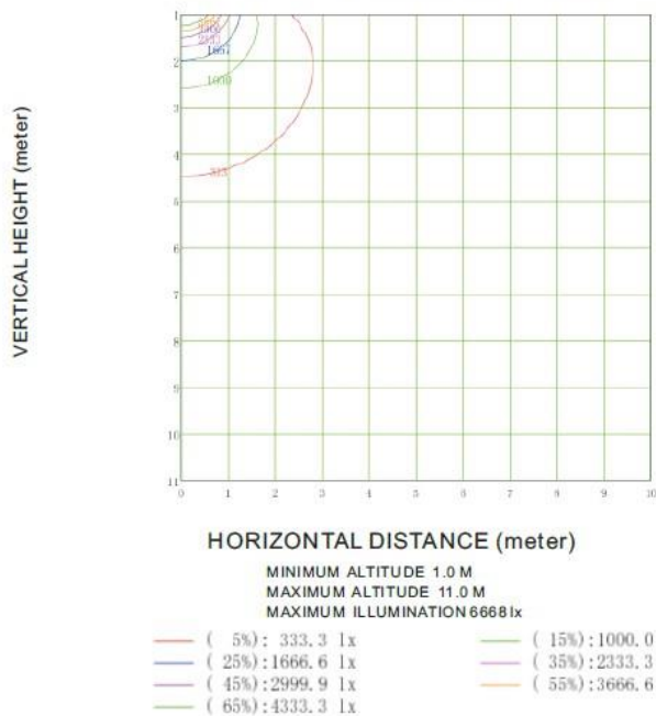
VERTICAL EQUILUMINOUS CURVE
